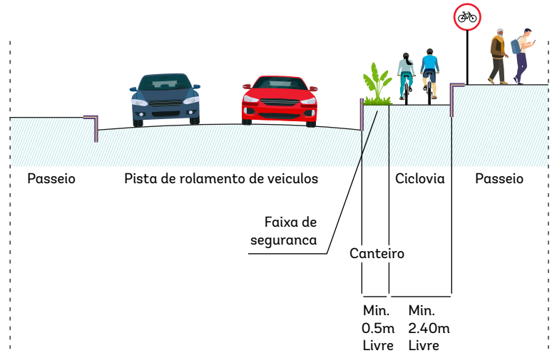
Figure 4.2. Example of street section with bidirectional, segregated cycle lane
